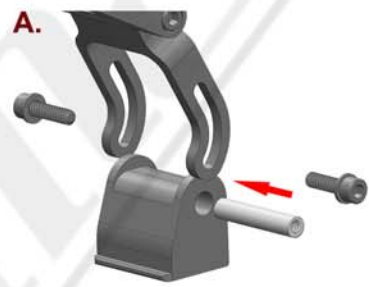
5 - Install aluminum threaded insert into magnet (fig A.), and attach magnet onto blindmount with lip pointed in direction as shown (fig B.).
